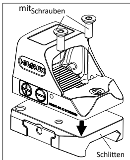
Abb. 4 Montage Picatinny-Adapter
